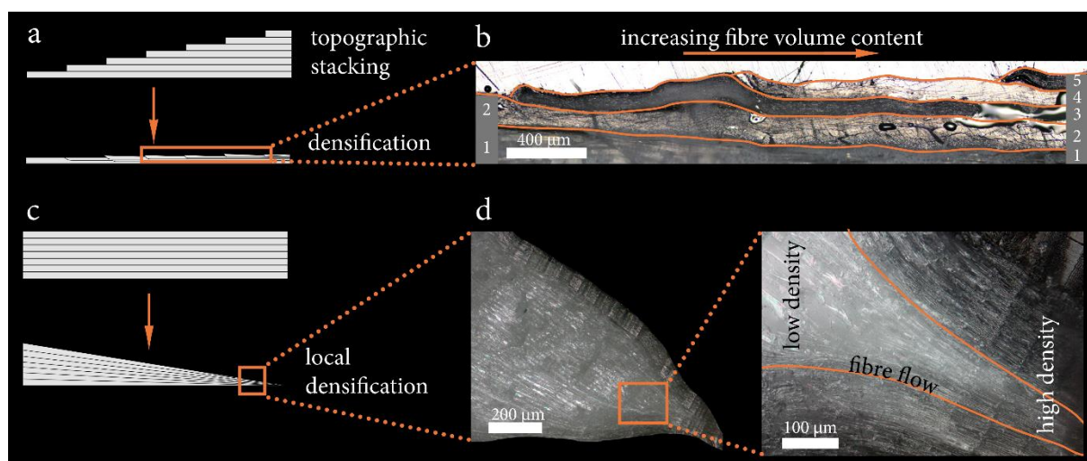
Figure 5. (a) Scheme of the topographic stacking method followed by densification. (b) Light-microscopy image of a topographically stacked material. The density is increased from left (2 layers) to right (5 layers). The layers are stacked 0/90° in order to distinguish the layers optically from each other. (c) Scheme of the local densification method. A stacked sample is densified into a wedge, which results in an increased density towards the tip. (d) Light-microscopy image (longitudinal cut) of delignified wood densified into a wedge.
