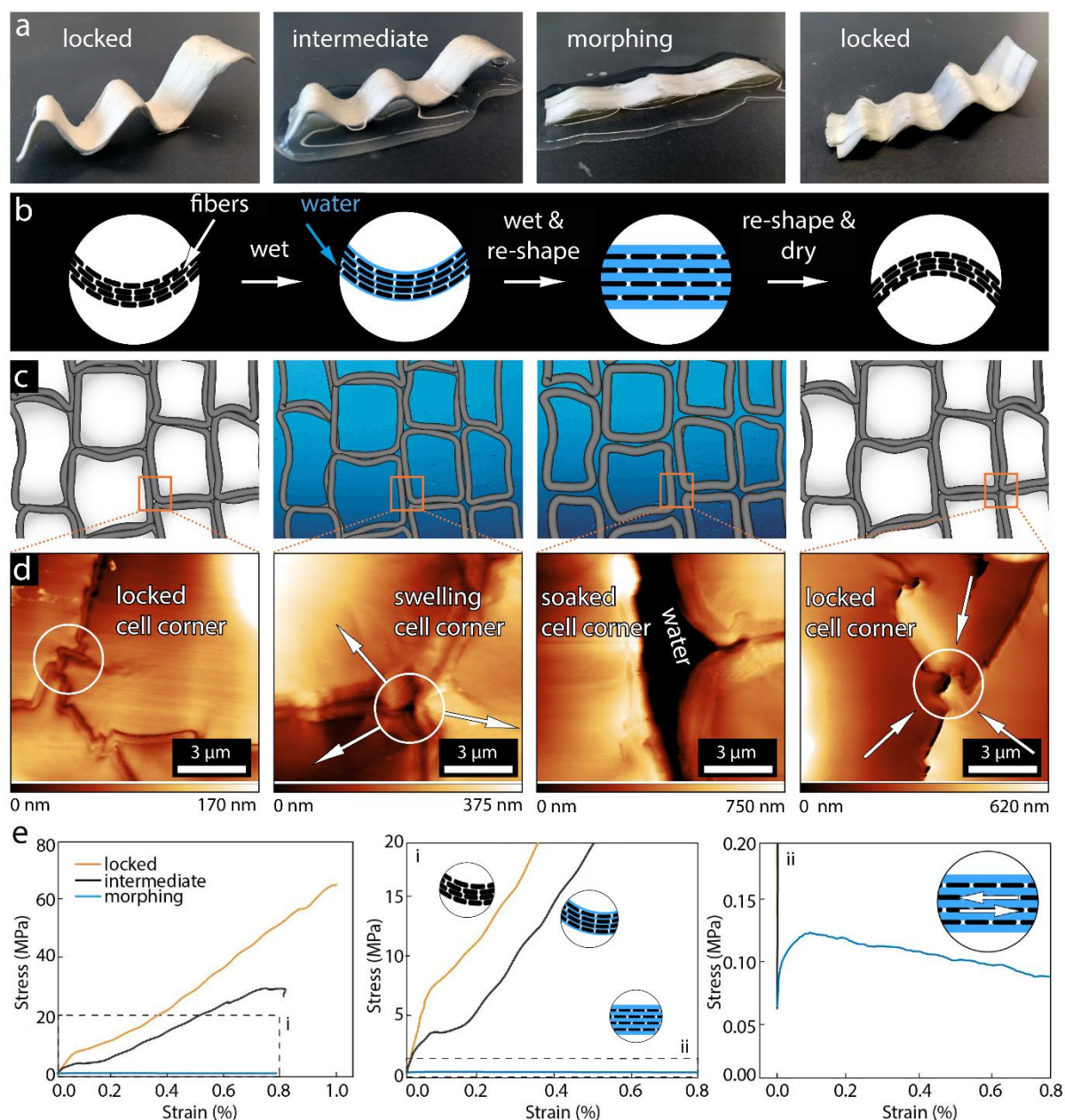
Figure 1. Shaping mechanism of delignified wood using moisture induced reversible interlocks. a) Delignified wood samples in the locked, intermediate, morphing and re-locked (after reshaping) state. b) Scheme of a longitudinal section of delignified wood in the four states, illustrating the swelling of delignified wood fibers (black) by water (blue). c) Scheme of a cross-section and (d) AFM images of the cell corner region showing the moisture induced interlocking mechanism. e) Representative tensile stress-strain curves of delignified wood in the locked (orange), intermediate (black) and morphing state (blue) and zoom into regions of interest (i,ii).
