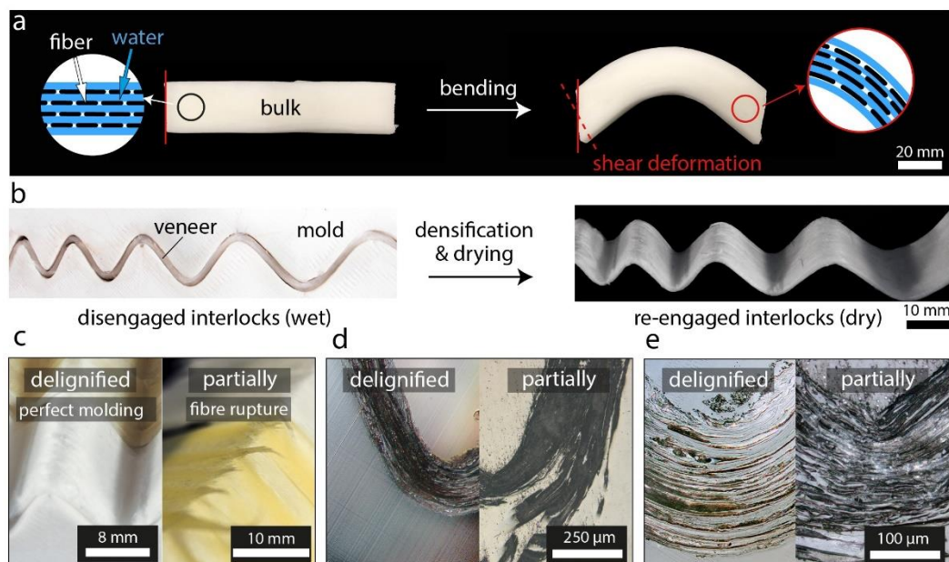
Figure 2. Bending of a delignified bulk wood sample in the morphing state results in (a) a shear deformed, curved sample. The sample shows vertically aligned edges (red line) after bending. The red dotted line illustrates the orthogonal to the neutral axes that would be expected for perfectly bonded interfaces. b) Densification of a delignified veneer in a cast ceramic mold followed by drying results in a stiff material due to the locked cell corners. c) Wet delignified wood drapes onto the mold while partially delignified wood veneers wrinkle and rupture. d), e) Light-microscope images of delignified and partially delignified veneers after densification in the mold demonstrate that complete removal of lignin is required to disengage mechanical interlocking of cell walls.
