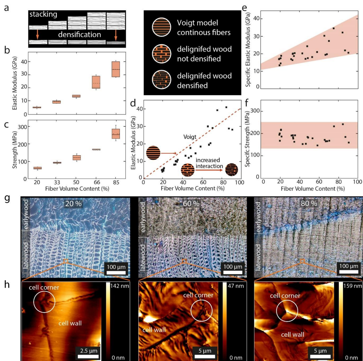
Figure 3. a) Stacking results in FVCs between 20% before densification up to values of 85% upon densification. b) Tensile elastic modulus and (c) strength versus normalized FVC demonstrate the broad range of properties that can be achieved. d) Elastic moduli compared to the Voigt model. e) Specific elastic modulus and (f) specific strength for FVCs between 20 and 85%. g) Light-microscope images show the densification behavior of delignified early- and
